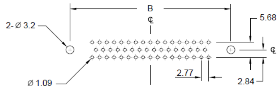
50 POSITIONS PCB LAYOUT
