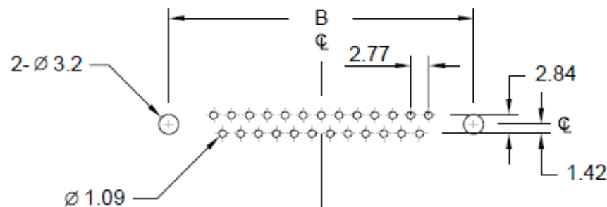
9, 15, 25, 37 POSITIONS PCB LAYOUT
